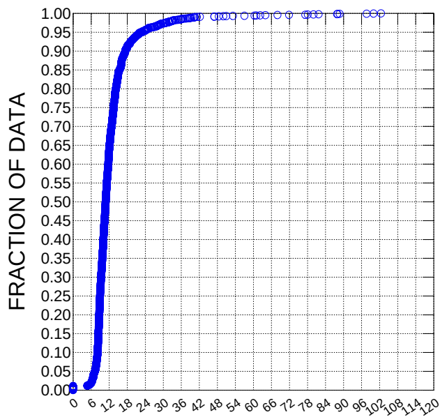
Figure 11b. Cumulative frequency flow plot for Sweetwater Branch with and without the Main Street WWTP
