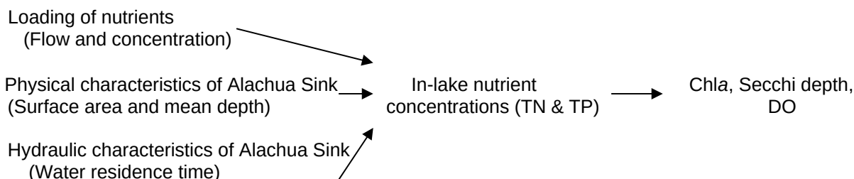
Figure 5. Bathtub conceptual scheme
